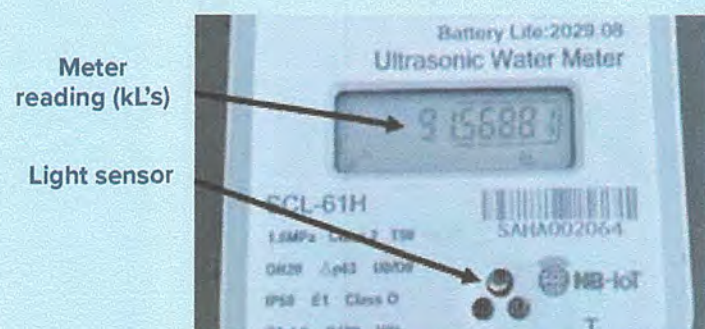
Example display shows a reading of 91.5kL
