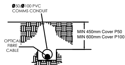
SECTION B-B BORE
