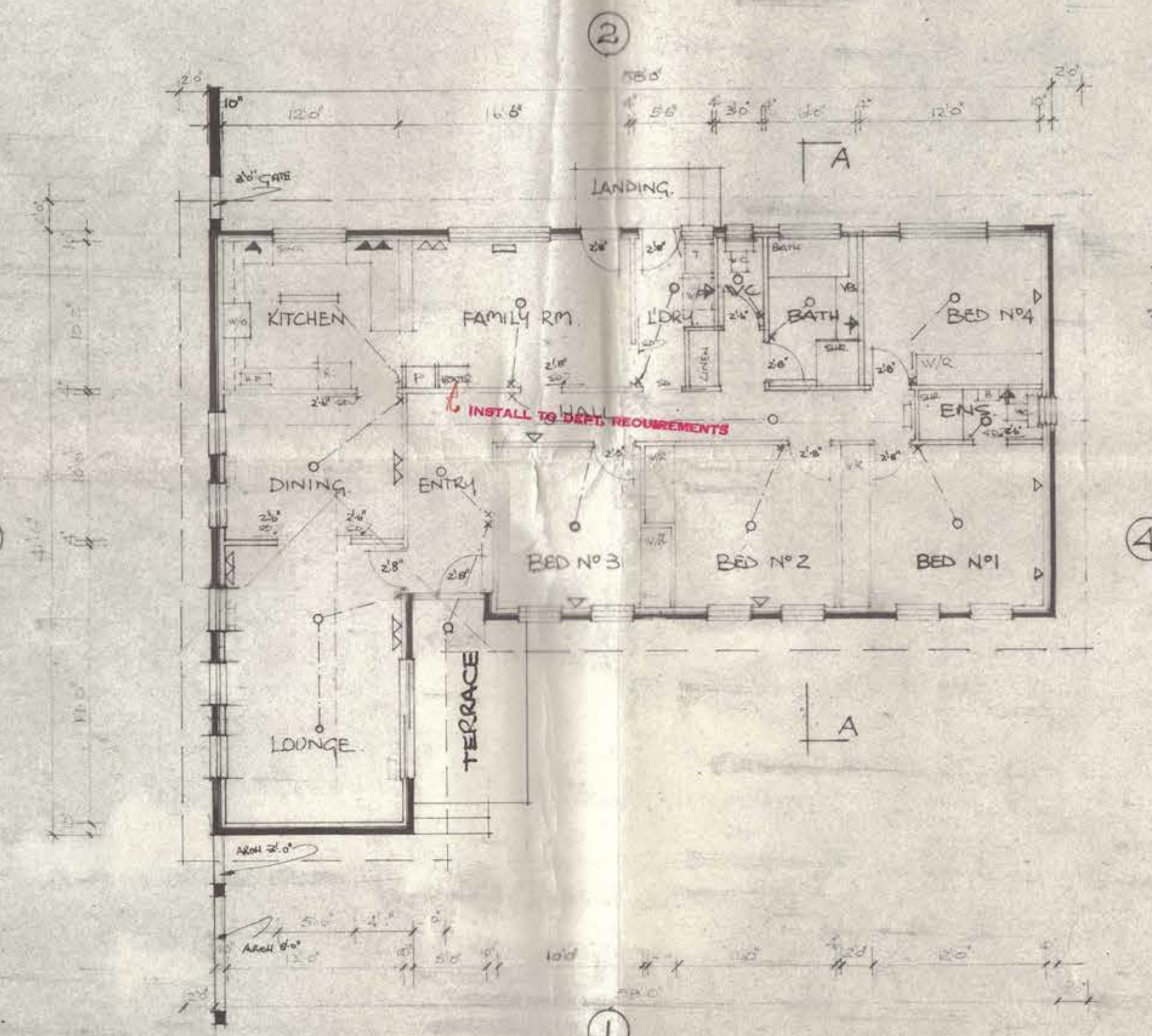
PLAN
