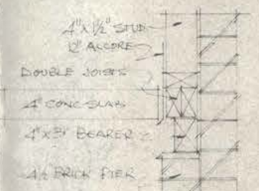
EXTERNAL WALL
